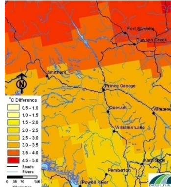
Winter Mean Temperature (2041 - 2070) Projection
