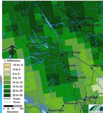
Winter Mean Precipitation (2041 - 2070) Projection
